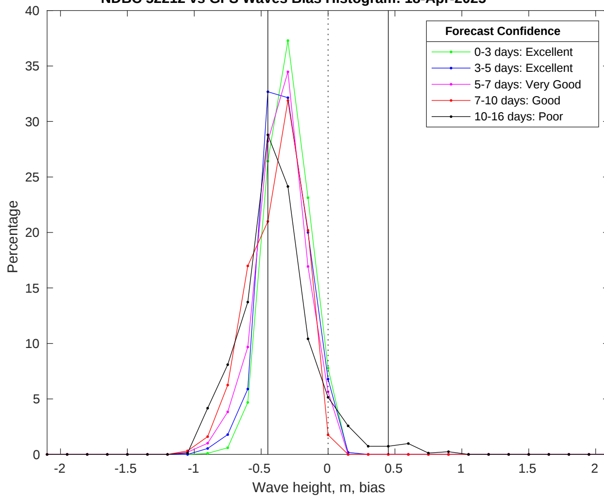
NDBC 52212 vs GFS Waves Bias Histogram: 18-Apr-2025
