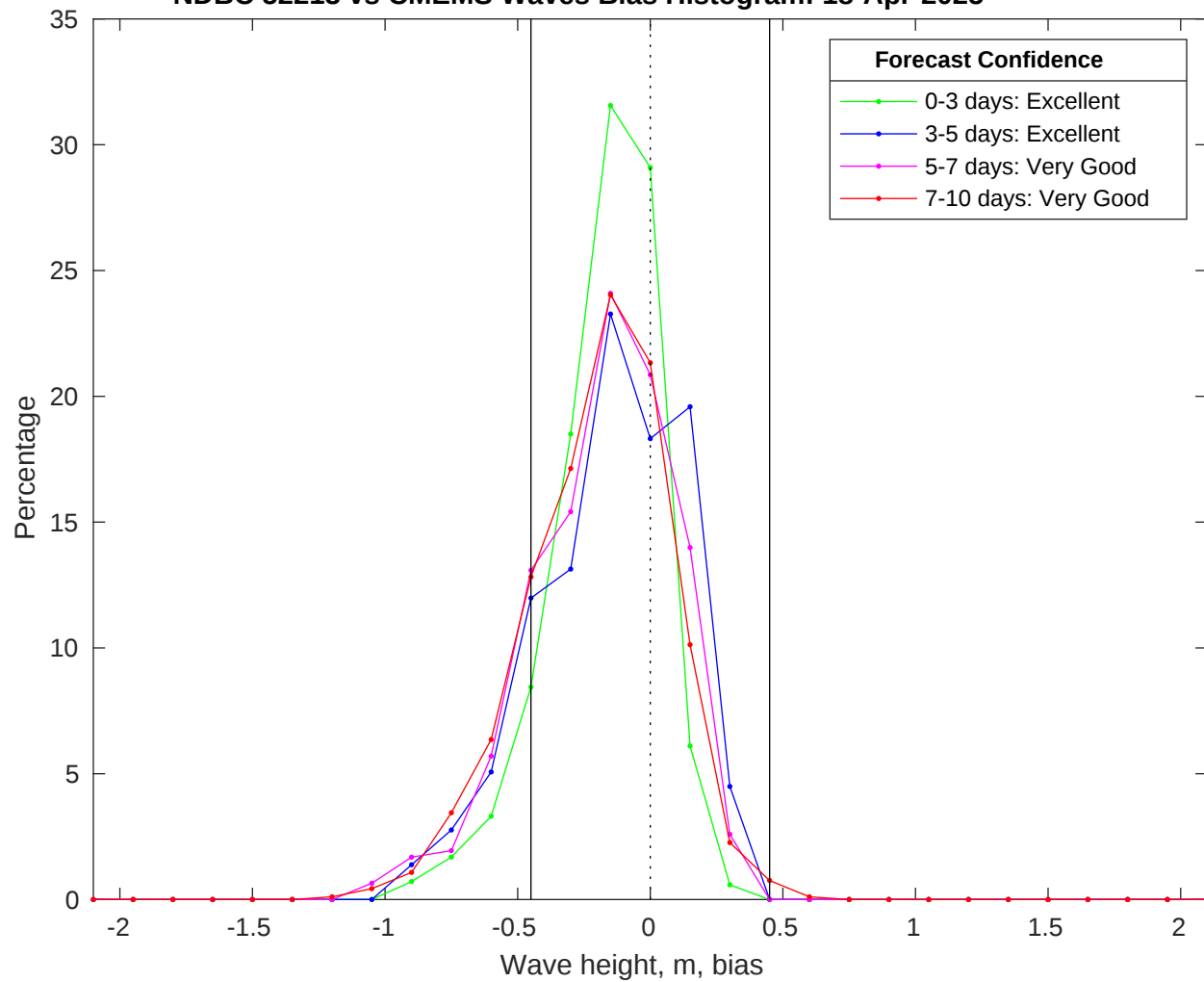
NDBC 52213 vs CMEMS Waves Bias Histogram: 18-Apr-2025
