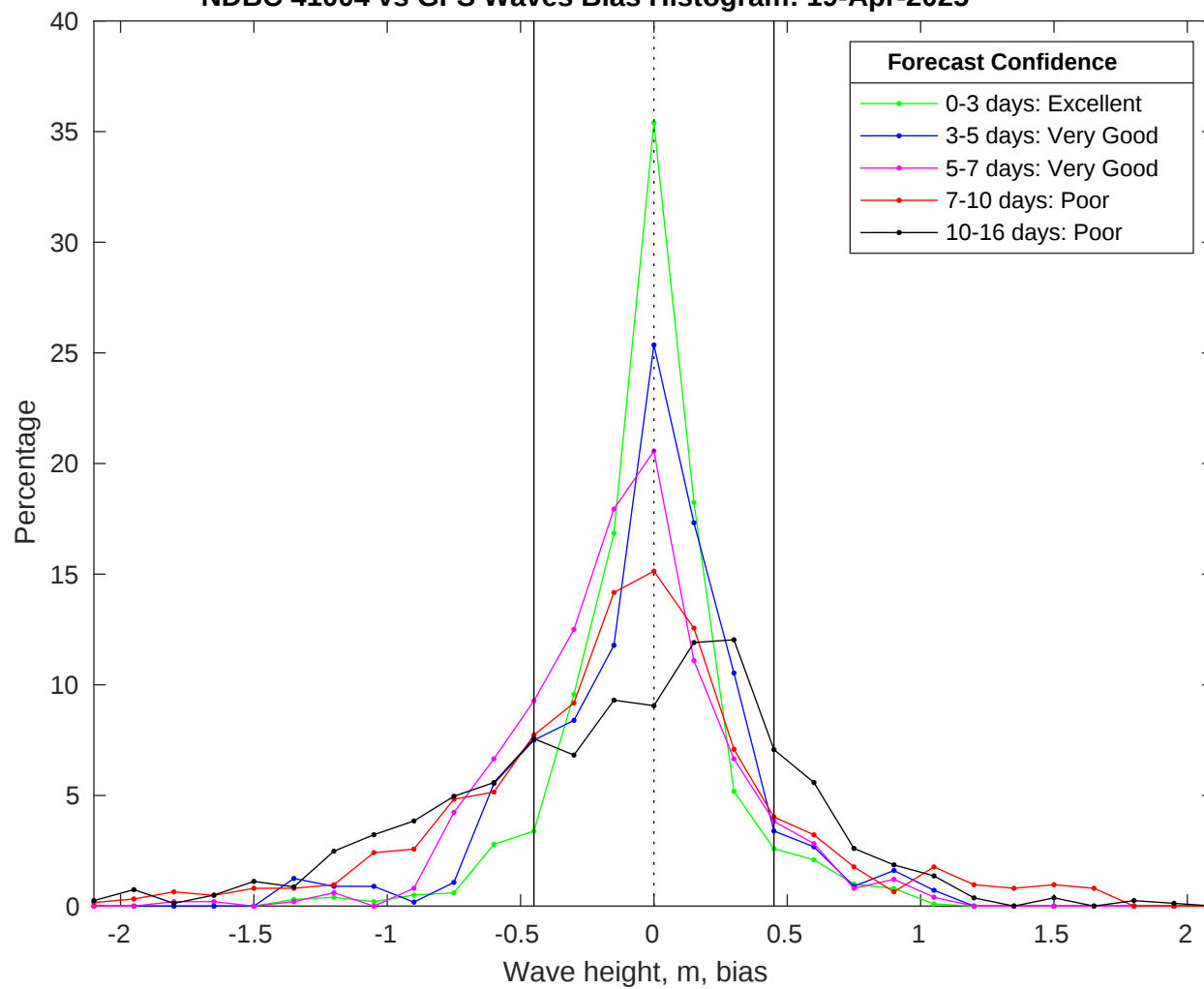
NDBC 41004 vs GFS Waves Bias Histogram: 19-Apr-2025
