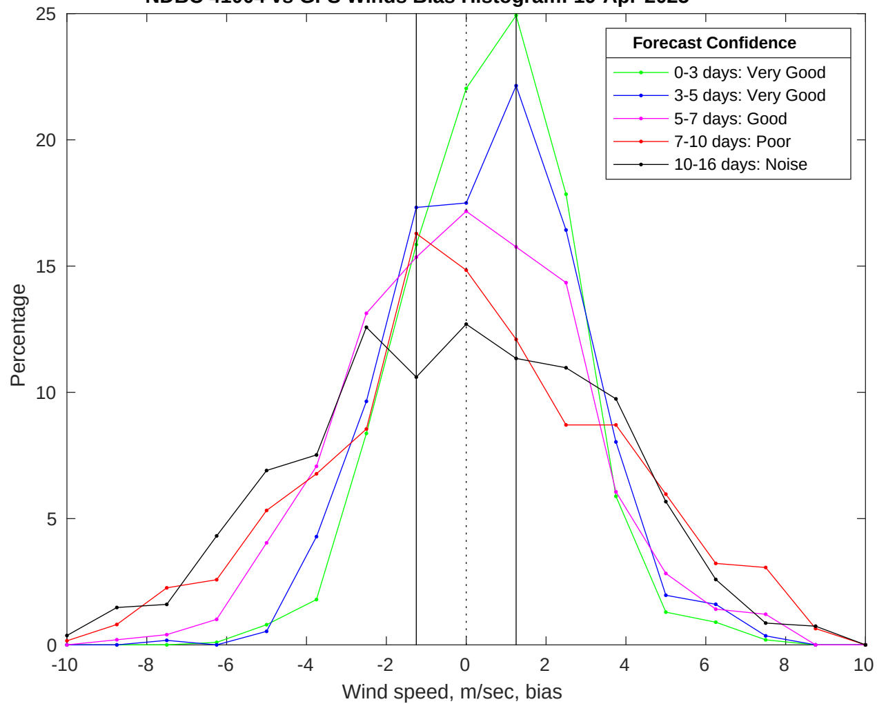
NDBC 41004 vs GFS Winds Bias Histogram: 19-Apr-2025
