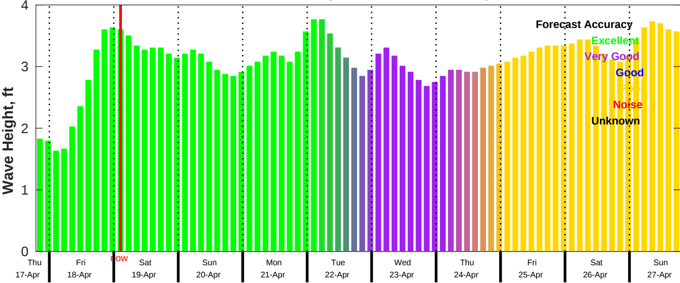
CMEMS Wave Forecast for NDBC 41004 from 17-Apr-2025 19:00:00 to 27-Apr-2025 19:00:00
