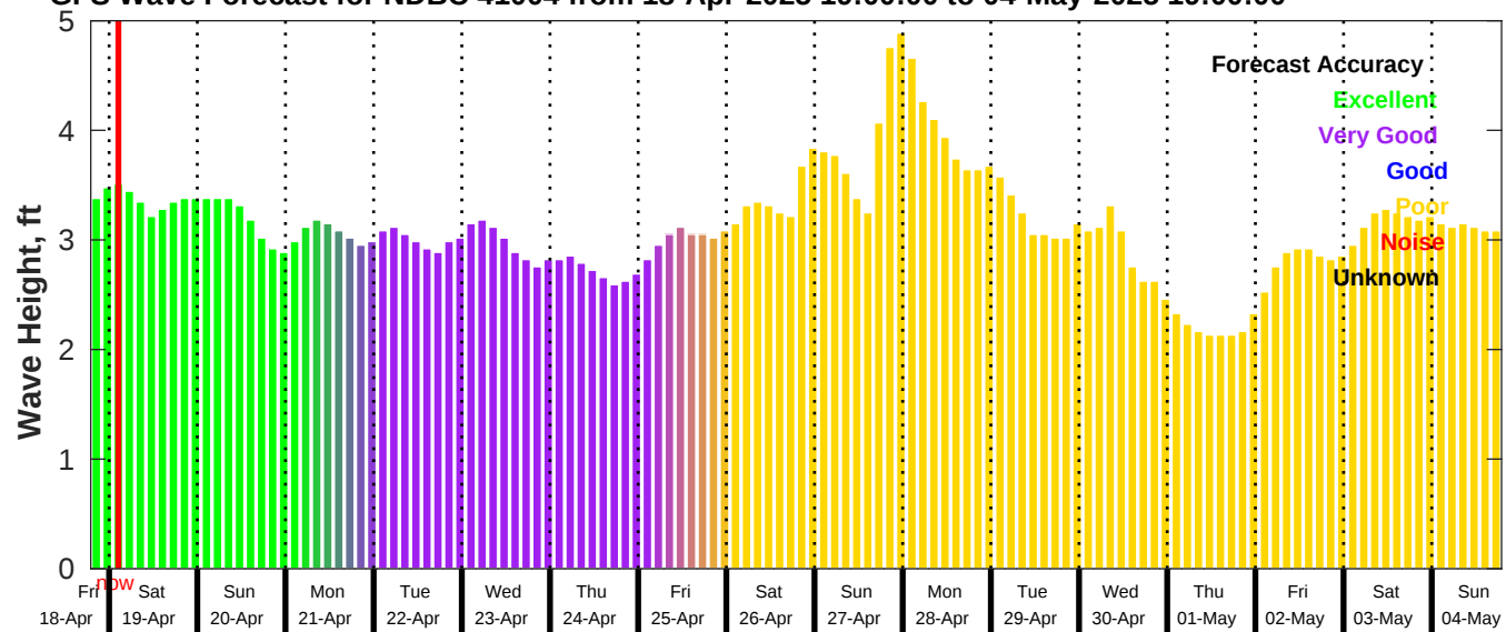
GFS Wave Forecast for NDBC 41004 from 18-Apr-2025 19:00:00 to 04-May-2025 19:00:00
