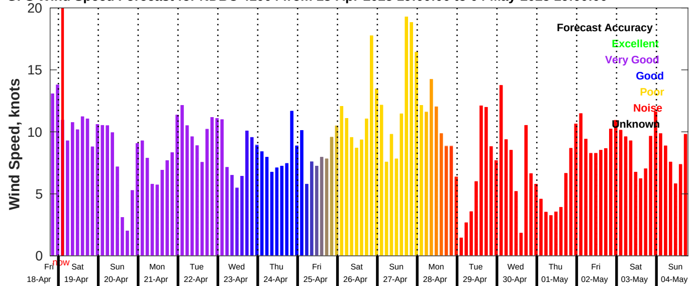
GFS Wind Speed Forecast for NDBC 41004 from 18-Apr-2025 19:00:00 to 04-May-2025 19:00:00
