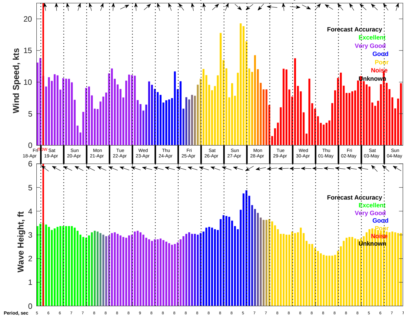
Wind & Wave Forecast for NDBC 41004 from 18-Apr-2025 19:00:00 to 04-May-2025 19:00:00
