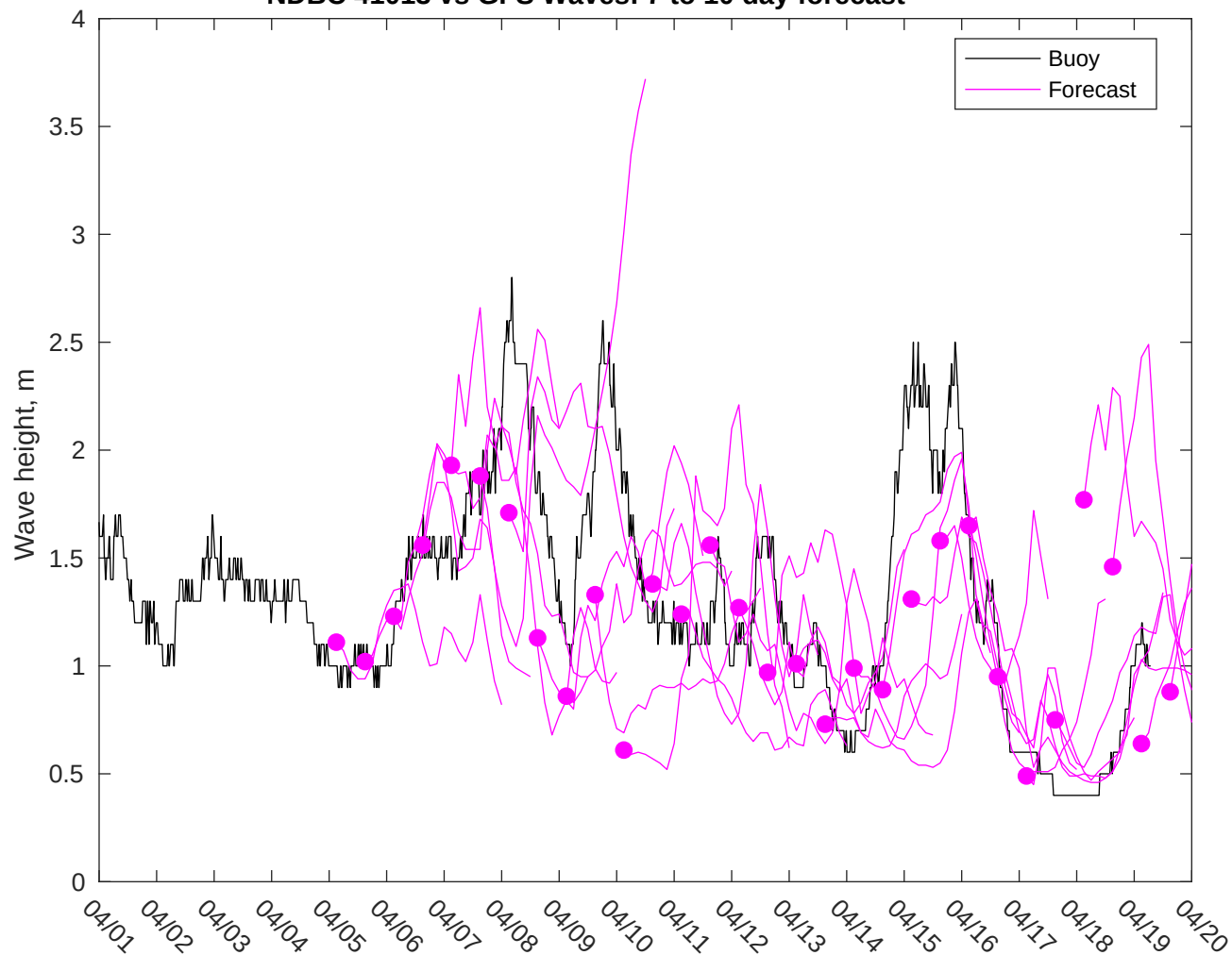
NDBC 41013 vs GFS Waves: 7 to 10 day forecast
