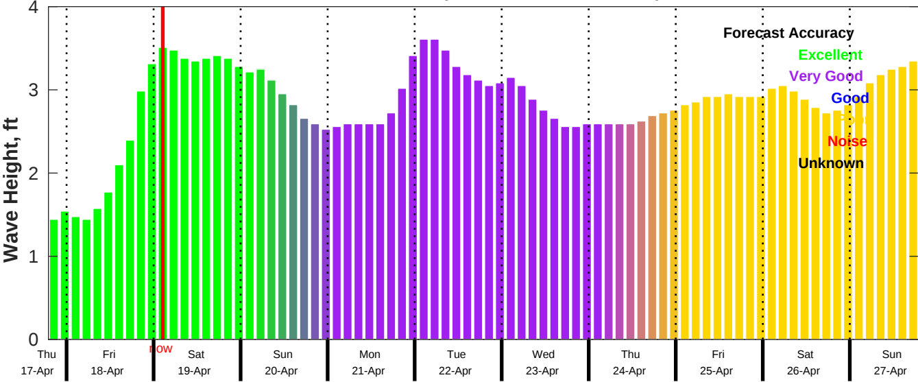
CMEMS Wave Forecast for NDBC 41013 from 17-Apr-2025 19:00:00 to 27-Apr-2025 19:00:00
