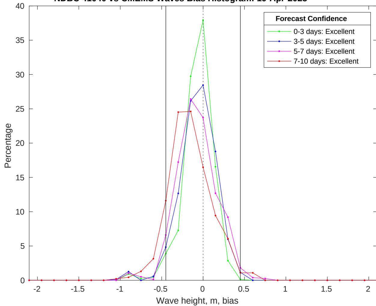
NDBC 41040 vs CMEMS Waves Bias Histogram: 19-Apr-2025
