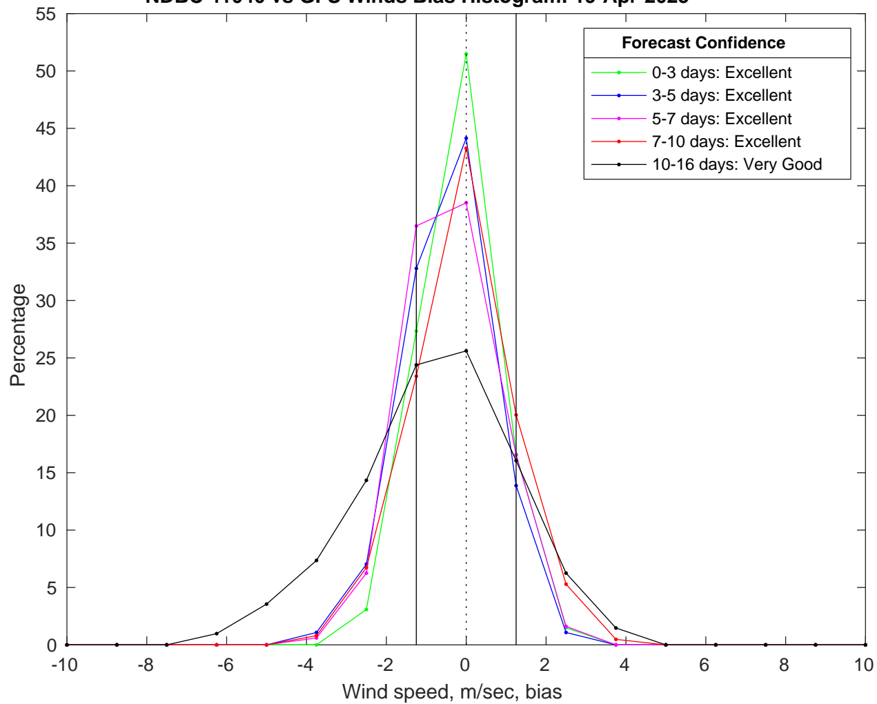
NDBC 41040 vs GFS Winds Bias Histogram: 19-Apr-2025
