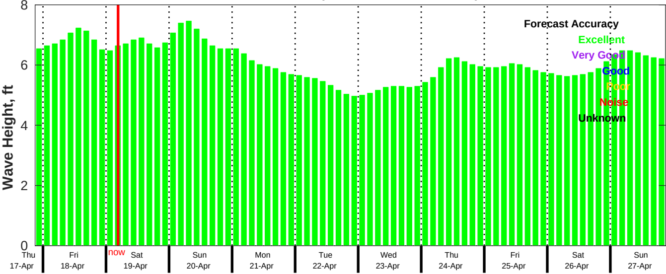
CMEMS Wave Forecast for NDBC 41040 from 17-Apr-2025 21:00:00 to 27-Apr-2025 21:00:00
