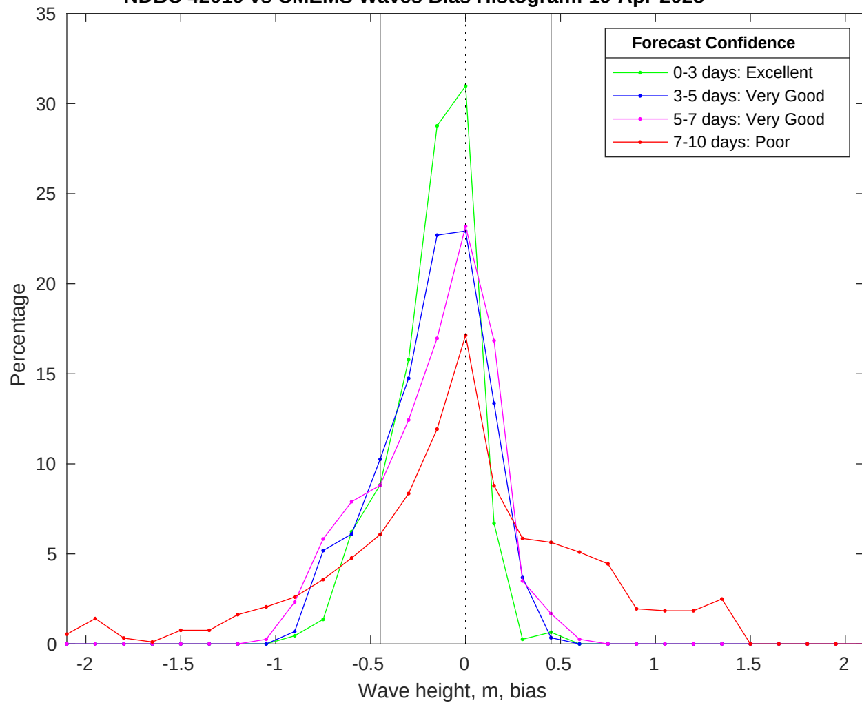
NDBC 42019 vs CMEMS Waves Bias Histogram: 19-Apr-2025
