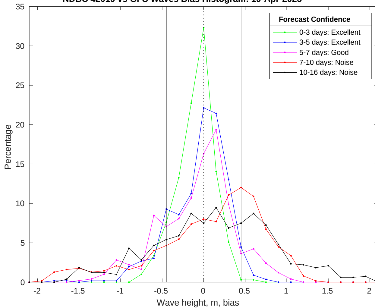
NDBC 42019 vs GFS Waves Bias Histogram: 19-Apr-2025
