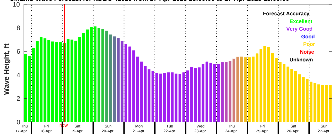
CMEMS Wave Forecast for NDBC 42019 from 17-Apr-2025 18:00:00 to 27-Apr-2025 18:00:00
