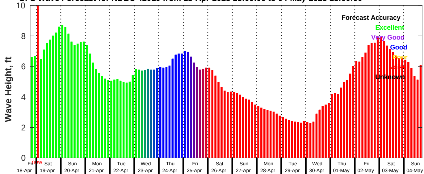
GFS Wave Forecast for NDBC 42019 from 18-Apr-2025 18:00:00 to 04-May-2025 18:00:00
