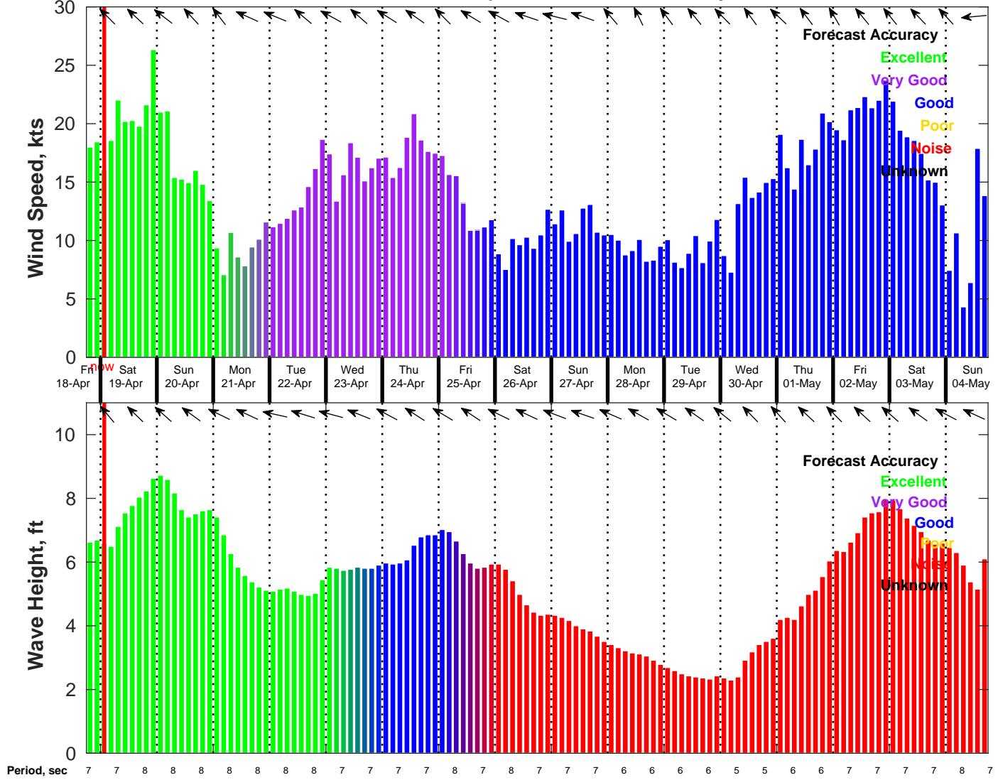
Wind & Wave Forecast for NDBC 42019 from 18-Apr-2025 18:00:00 to 04-May-2025 18:00:00
