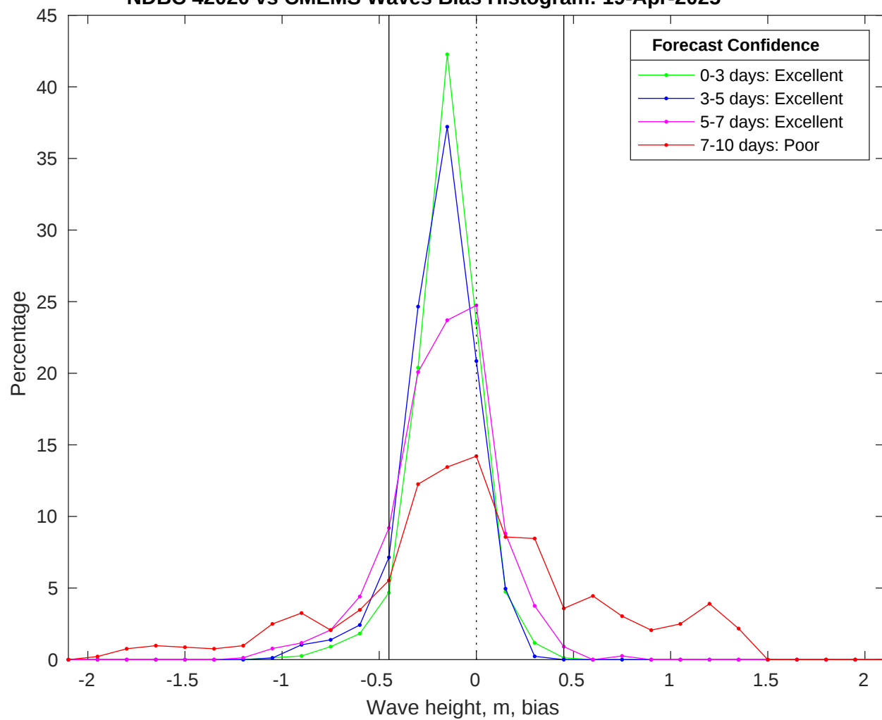
NDBC 42020 vs CMEMS Waves Bias Histogram: 19-Apr-2025
