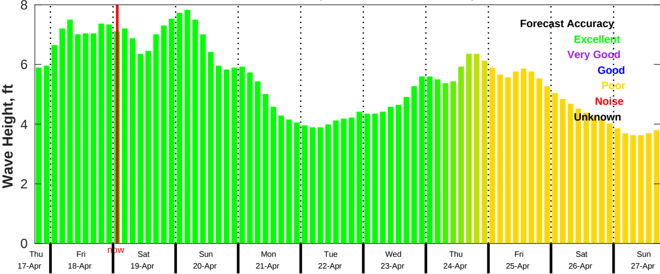
CMEMS Wave Forecast for NDBC 42020 from 17-Apr-2025 18:00:00 to 27-Apr-2025 18:00:00
