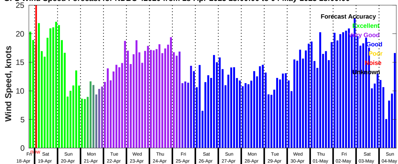
GFS Wind Speed Forecast for NDBC 42020 from 18-Apr-2025 18:00:00 to 04-May-2025 18:00:00
