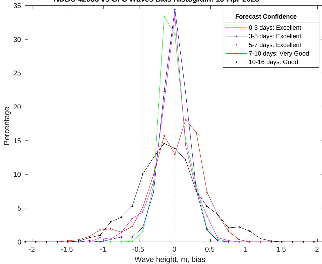
NDBC 42035 vs GFS Waves Bias Histogram: 19-Apr-2025
