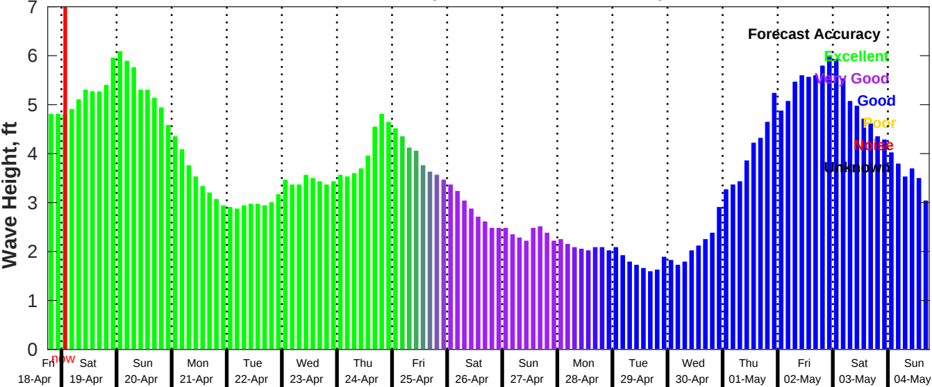
GFS Wave Forecast for NDBC 42035 from 18-Apr-2025 18:00:00 to 04-May-2025 18:00:00
