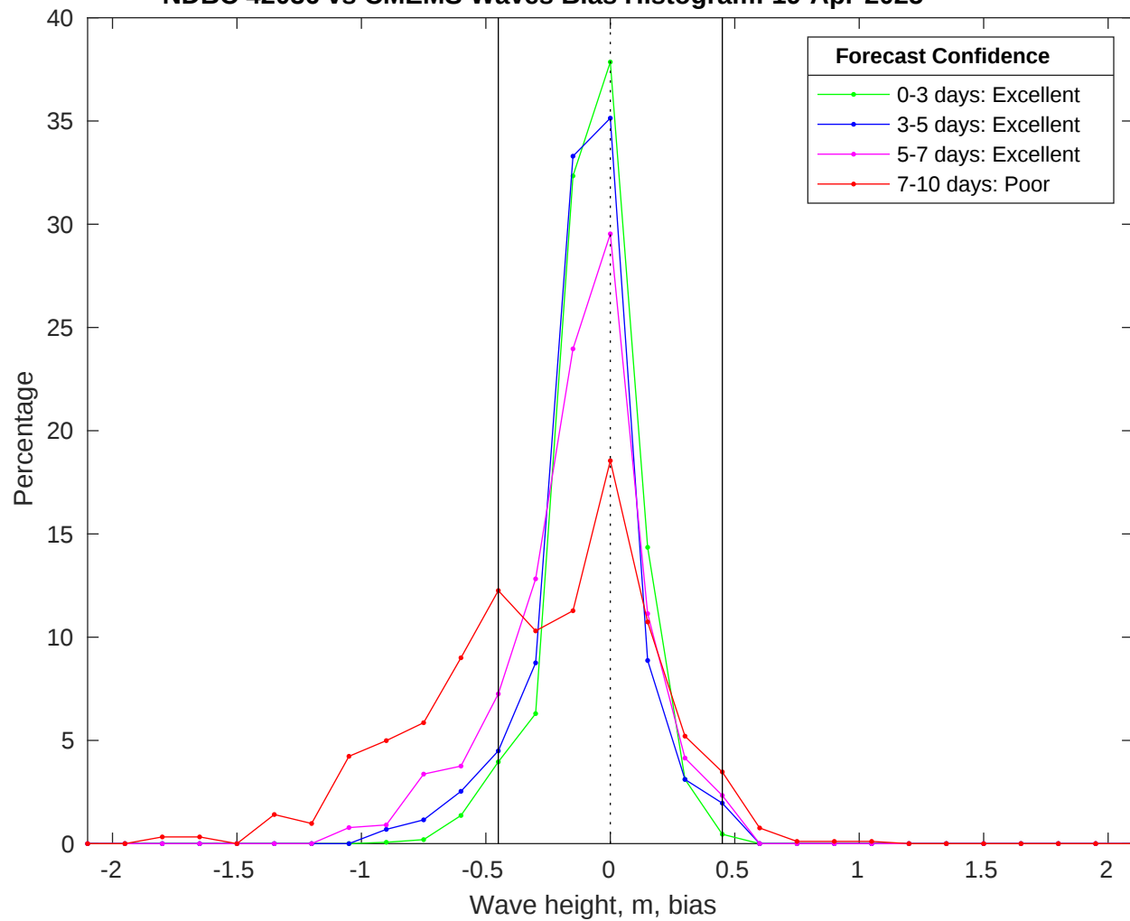
NDBC 42036 vs CMEMS Waves Bias Histogram: 19-Apr-2025
