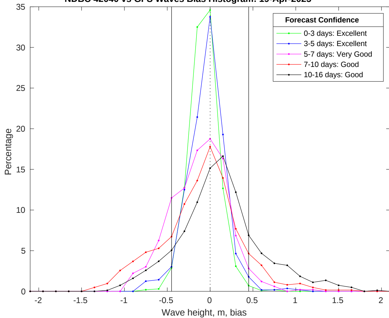
NDBC 42040 vs GFS Waves Bias Histogram: 19-Apr-2025
