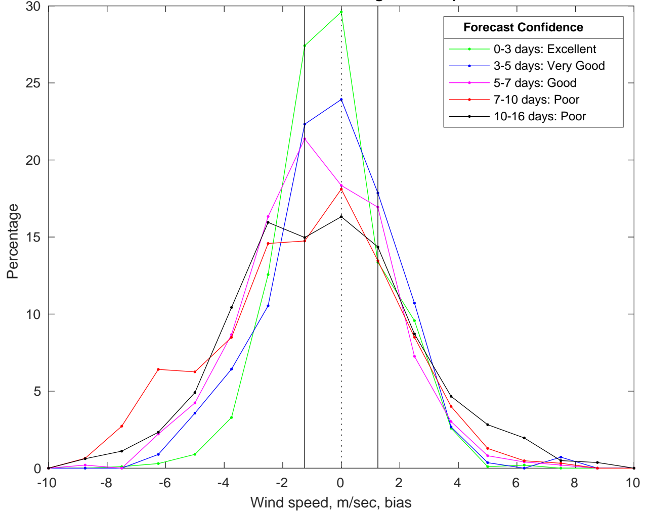
NDBC 42040 vs GFS Winds Bias Histogram: 19-Apr-2025
