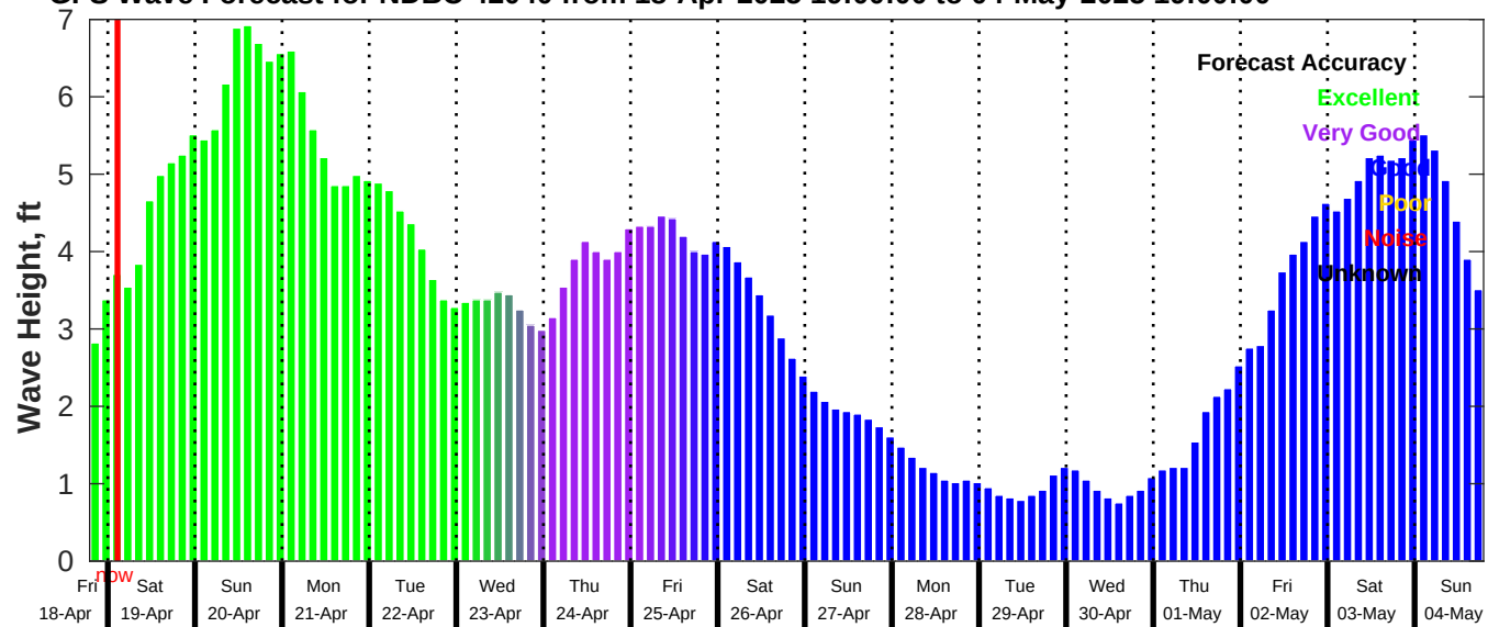
GFS Wave Forecast for NDBC 42040 from 18-Apr-2025 19:00:00 to 04-May-2025 19:00:00
