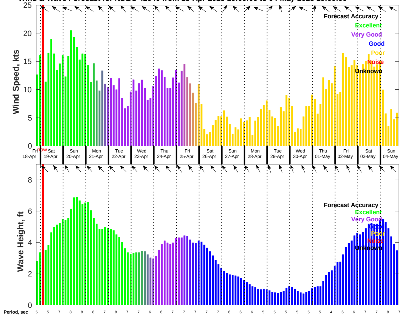
Wind & Wave Forecast for NDBC 42040 from 18-Apr-2025 19:00:00 to 04-May-2025 19:00:00
