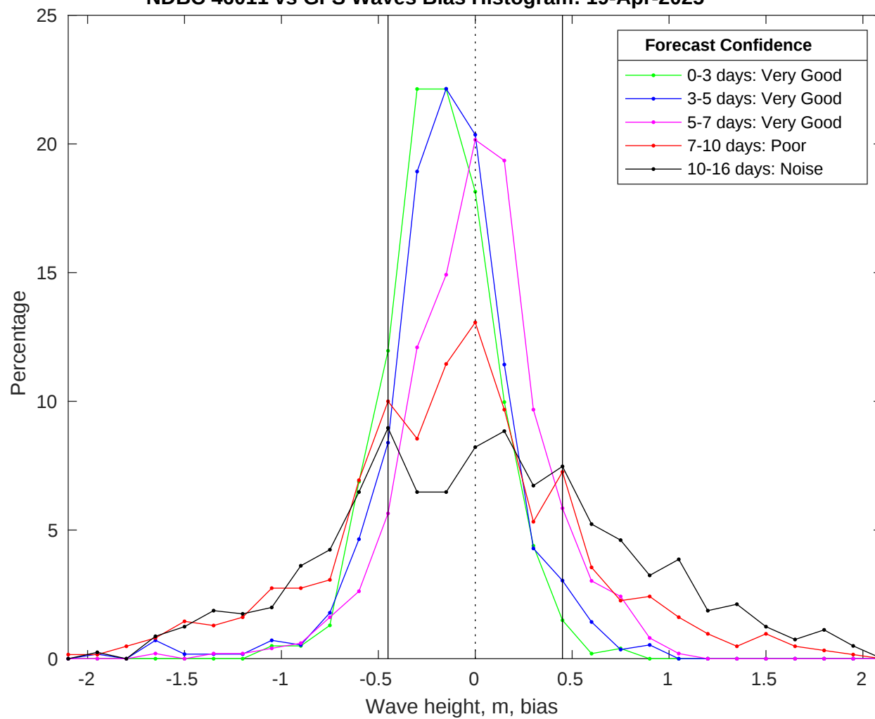
NDBC 46011 vs GFS Waves Bias Histogram: 19-Apr-2025
