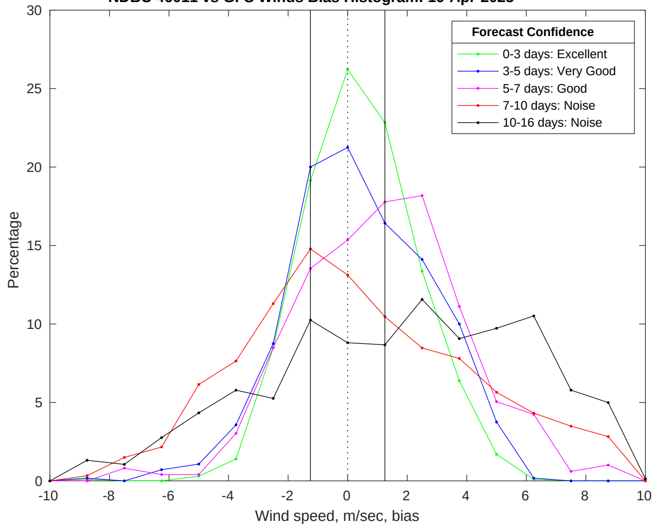
NDBC 46011 vs GFS Winds Bias Histogram: 19-Apr-2025
