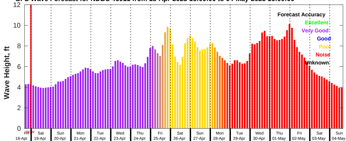
GFS Wave Forecast for NDBC 46011 from 18-Apr-2025 16:00:00 to 04-May-2025 16:00:00
