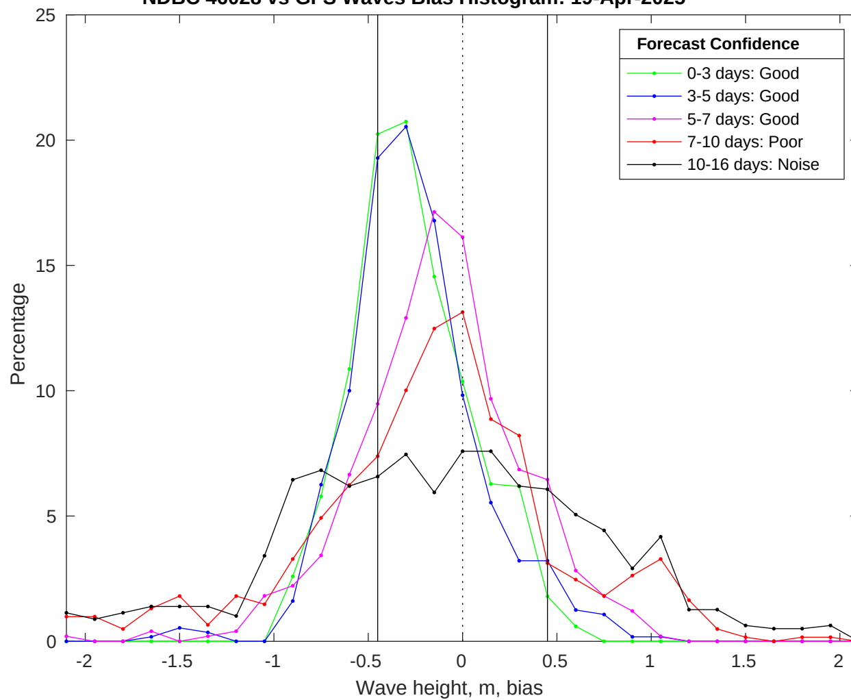
NDBC 46028 vs GFS Waves Bias Histogram: 19-Apr-2025
