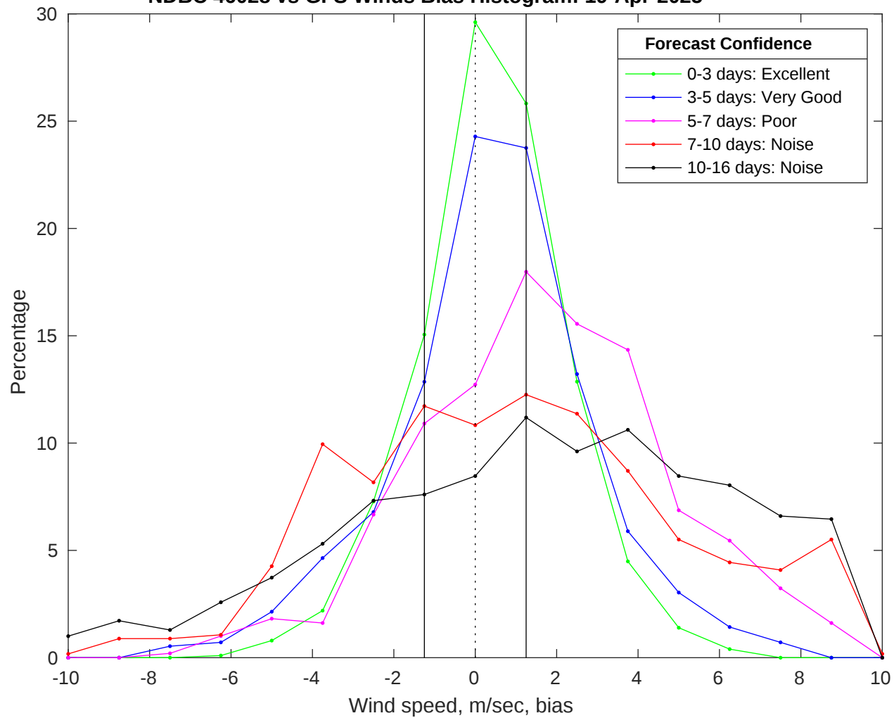
NDBC 46028 vs GFS Winds Bias Histogram: 19-Apr-2025
