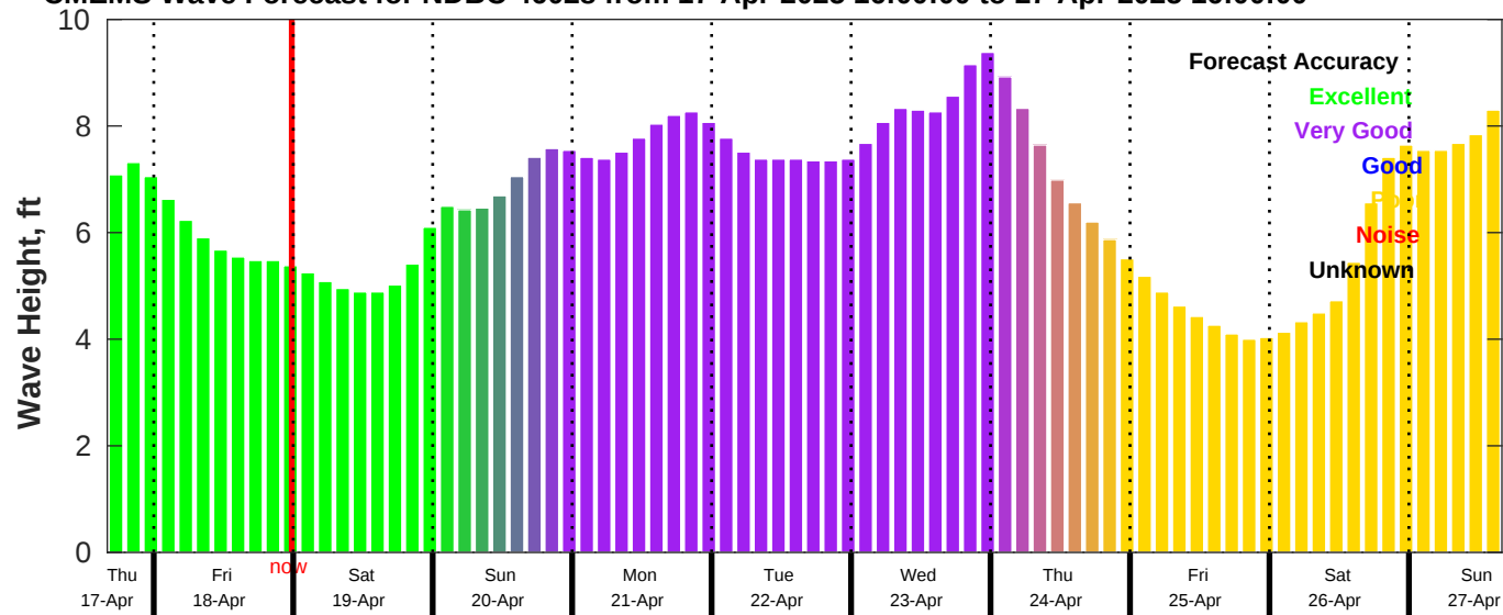
CMEMS Wave Forecast for NDBC 46028 from 17-Apr-2025 16:00:00 to 27-Apr-2025 16:00:00
