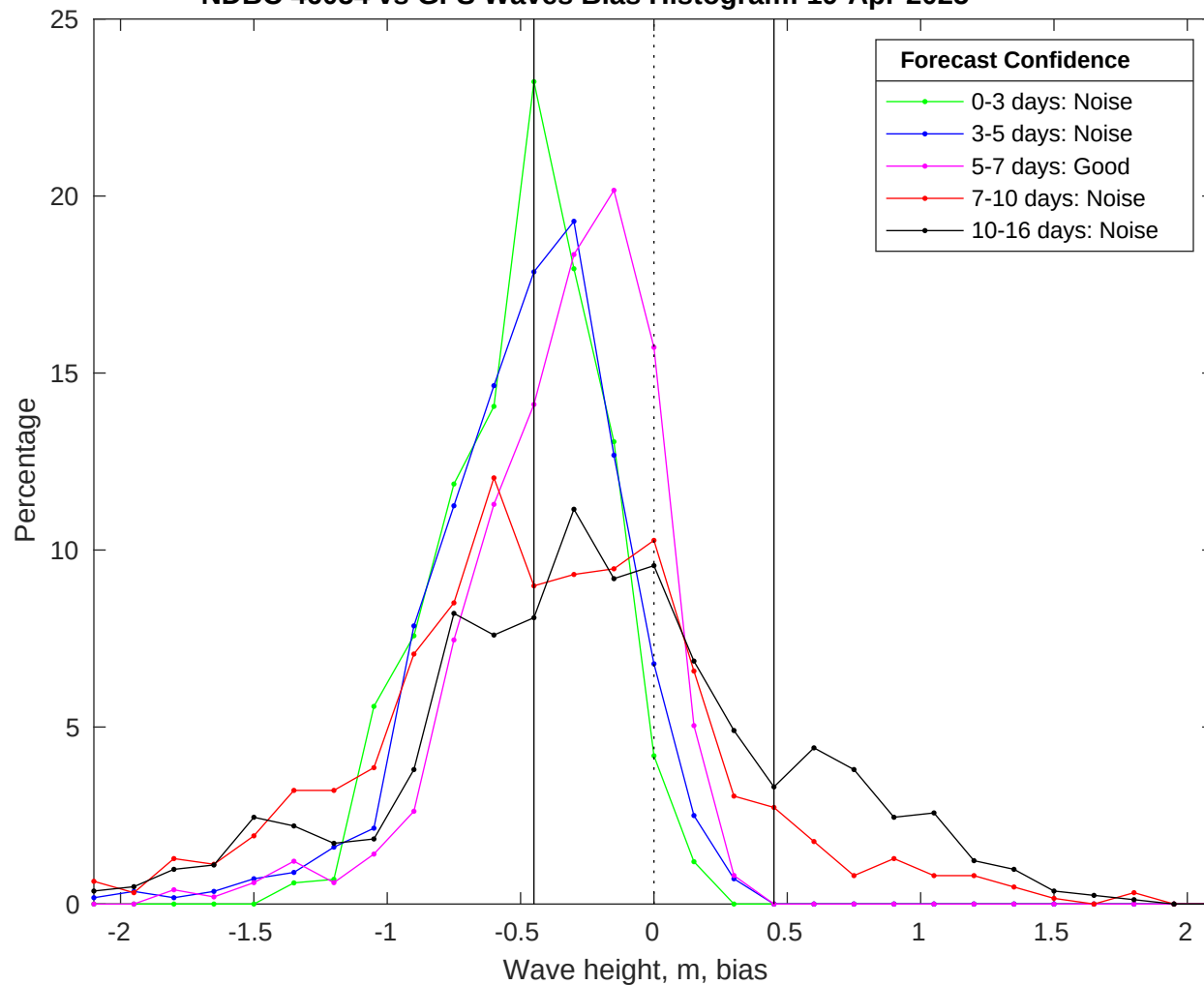
NDBC 46054 vs GFS Waves Bias Histogram: 19-Apr-2025
