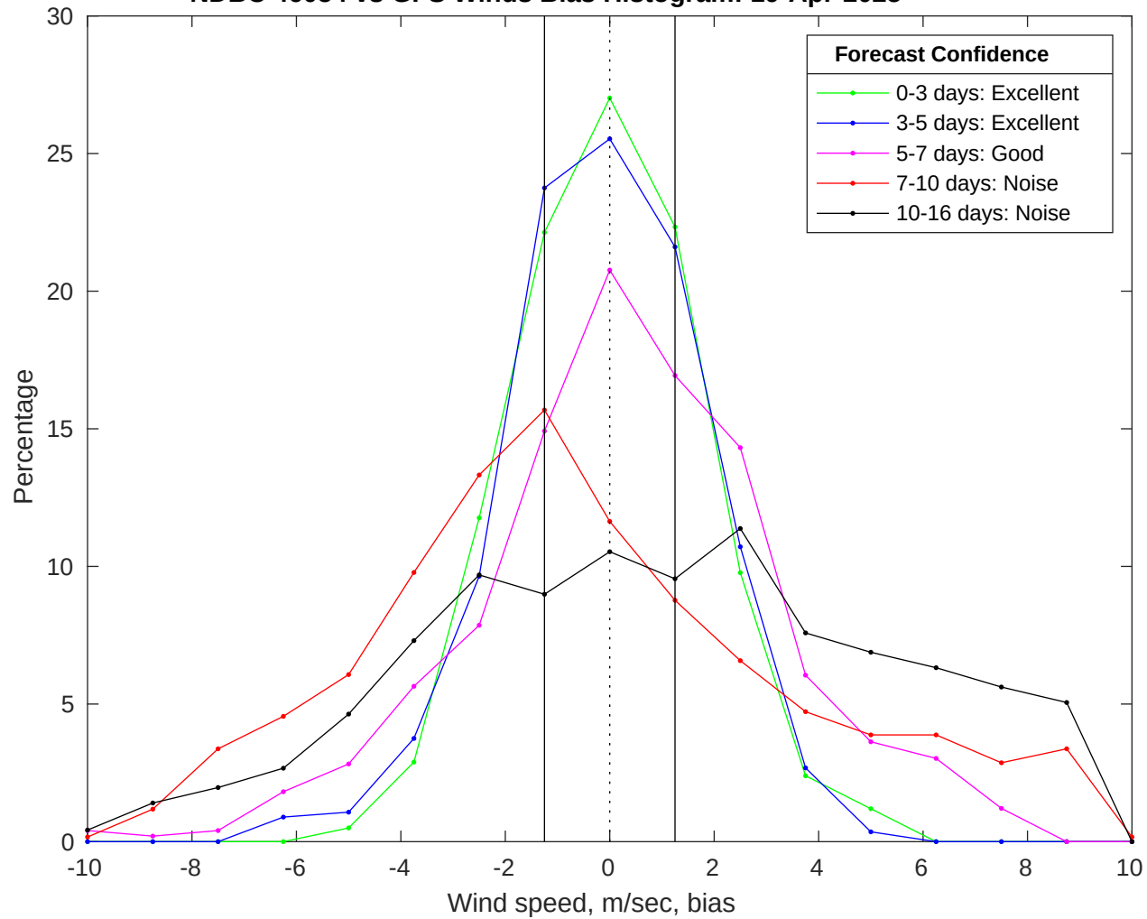
NDBC 46054 vs GFS Winds Bias Histogram: 19-Apr-2025
