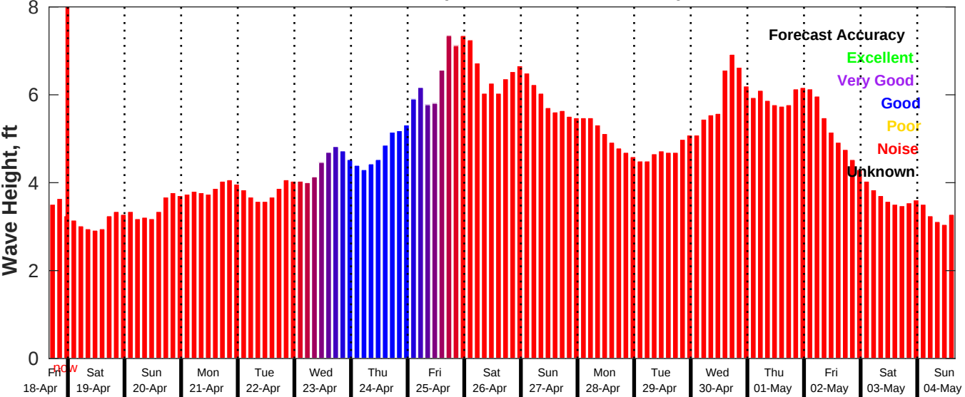
GFS Wave Forecast for NDBC 46054 from 18-Apr-2025 16:00:00 to 04-May-2025 16:00:00
