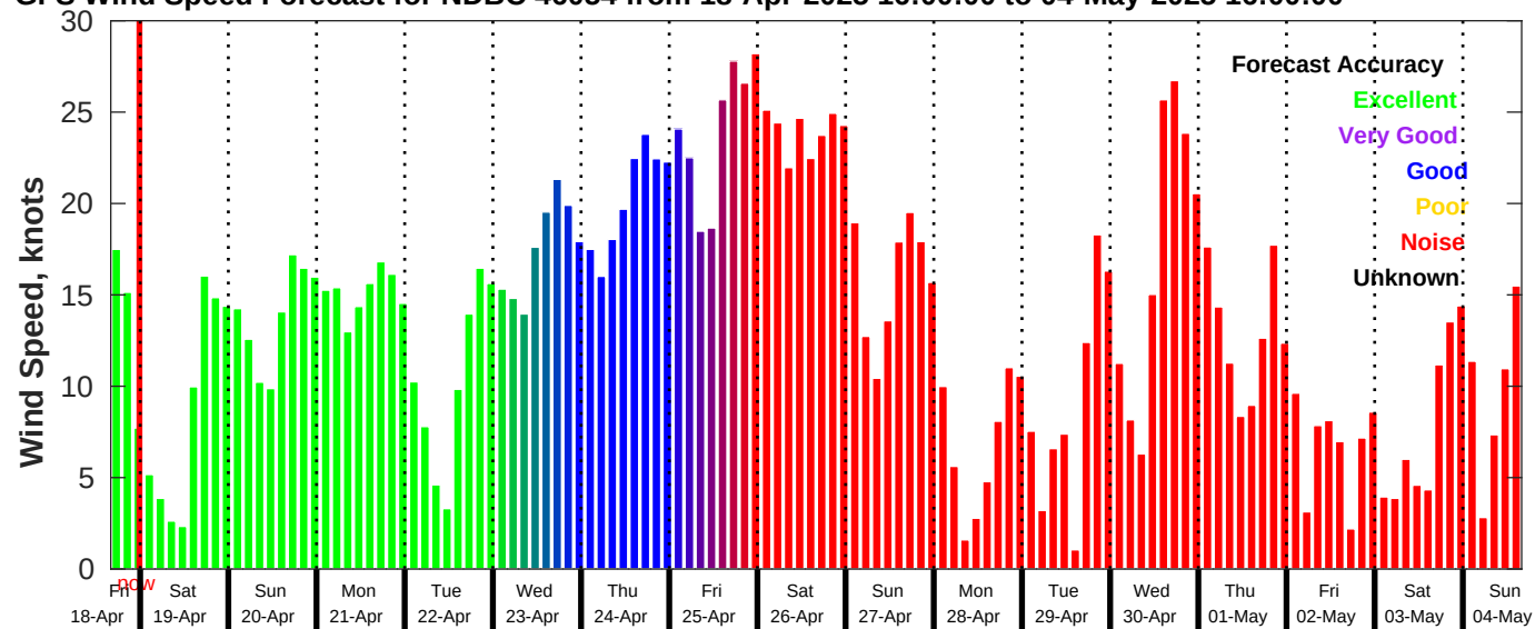
GFS Wind Speed Forecast for NDBC 46054 from 18-Apr-2025 16:00:00 to 04-May-2025 16:00:00
