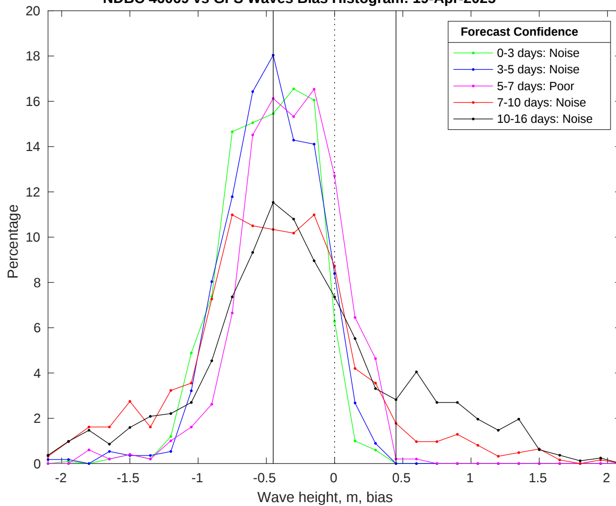
NDBC 46069 vs GFS Waves Bias Histogram: 19-Apr-2025
