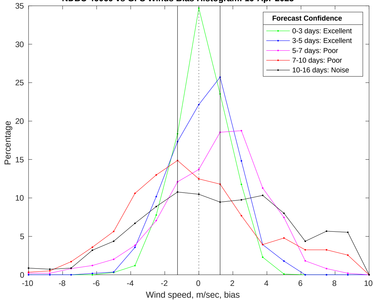
NDBC 46069 vs GFS Winds Bias Histogram: 19-Apr-2025
