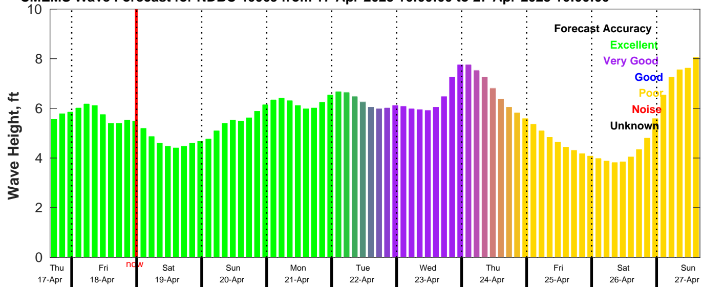
CMEMS Wave Forecast for NDBC 46069 from 17-Apr-2025 16:00:00 to 27-Apr-2025 16:00:00
