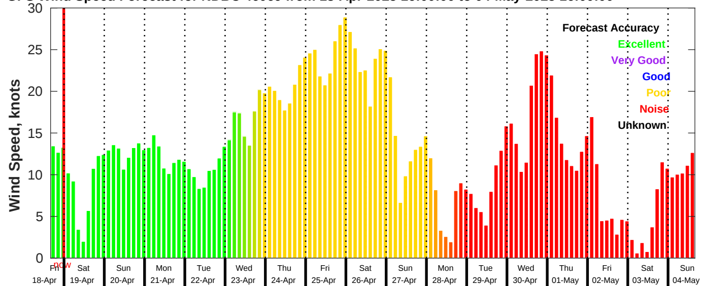
GFS Wind Speed Forecast for NDBC 46069 from 18-Apr-2025 16:00:00 to 04-May-2025 16:00:00
