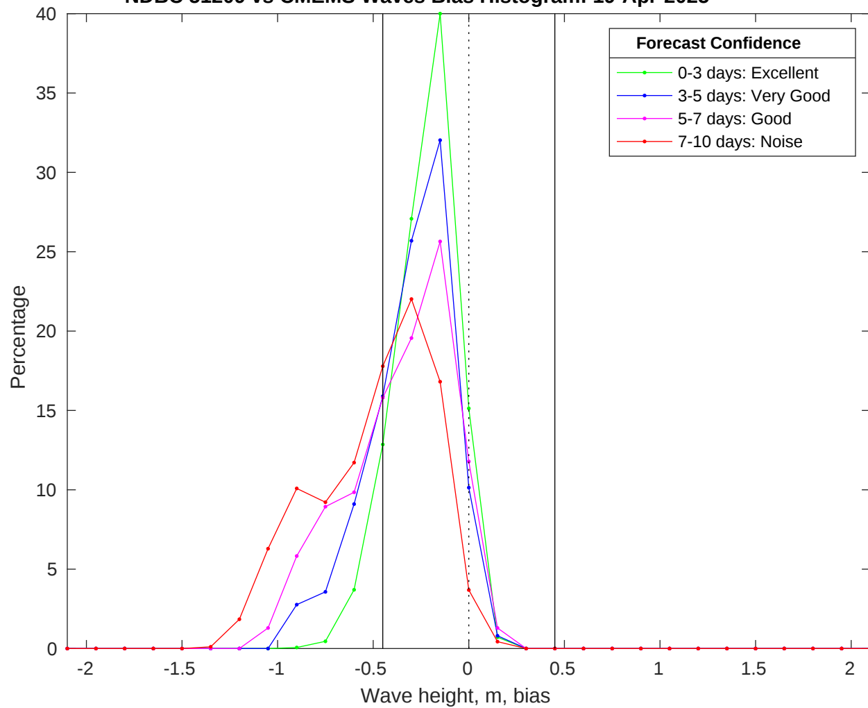
NDBC 51209 vs CMEMS Waves Bias Histogram: 19-Apr-2025
