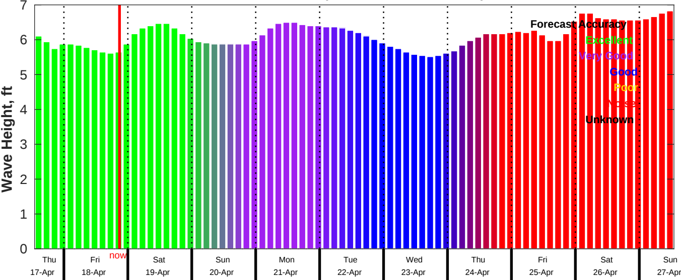
CMEMS Wave Forecast for NDBC 51209 from 17-Apr-2025 13:00:00 to 27-Apr-2025 13:00:00
