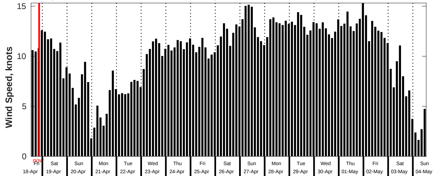
GFS Wind Speed Forecast for NDBC 51209 from 18-Apr-2025 13:00:00 to 04-May-2025 13:00:00
