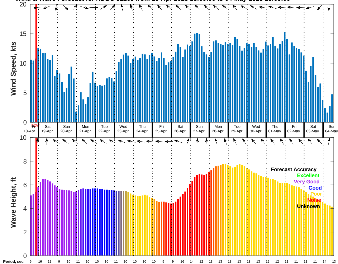
Wind & Wave Forecast for NDBC 51209 from 18-Apr-2025 13:00:00 to 04-May-2025 13:00:00
