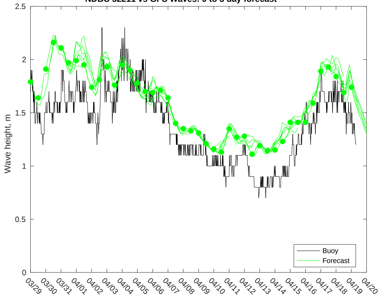
NDBC 52211 vs GFS Waves: 0 to 3 day forecast
