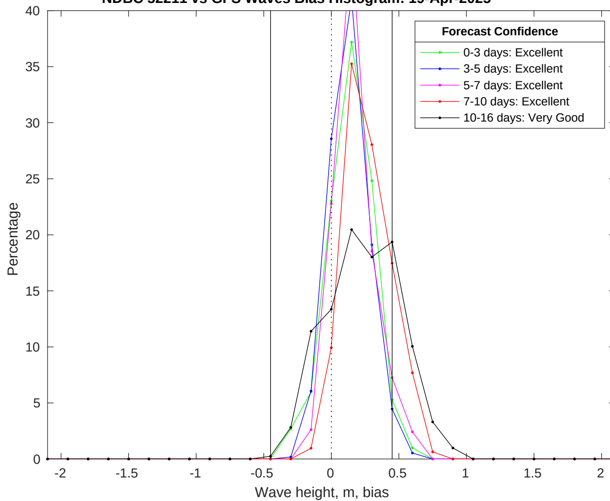
NDBC 52211 vs GFS Waves Bias Histogram: 19-Apr-2025
