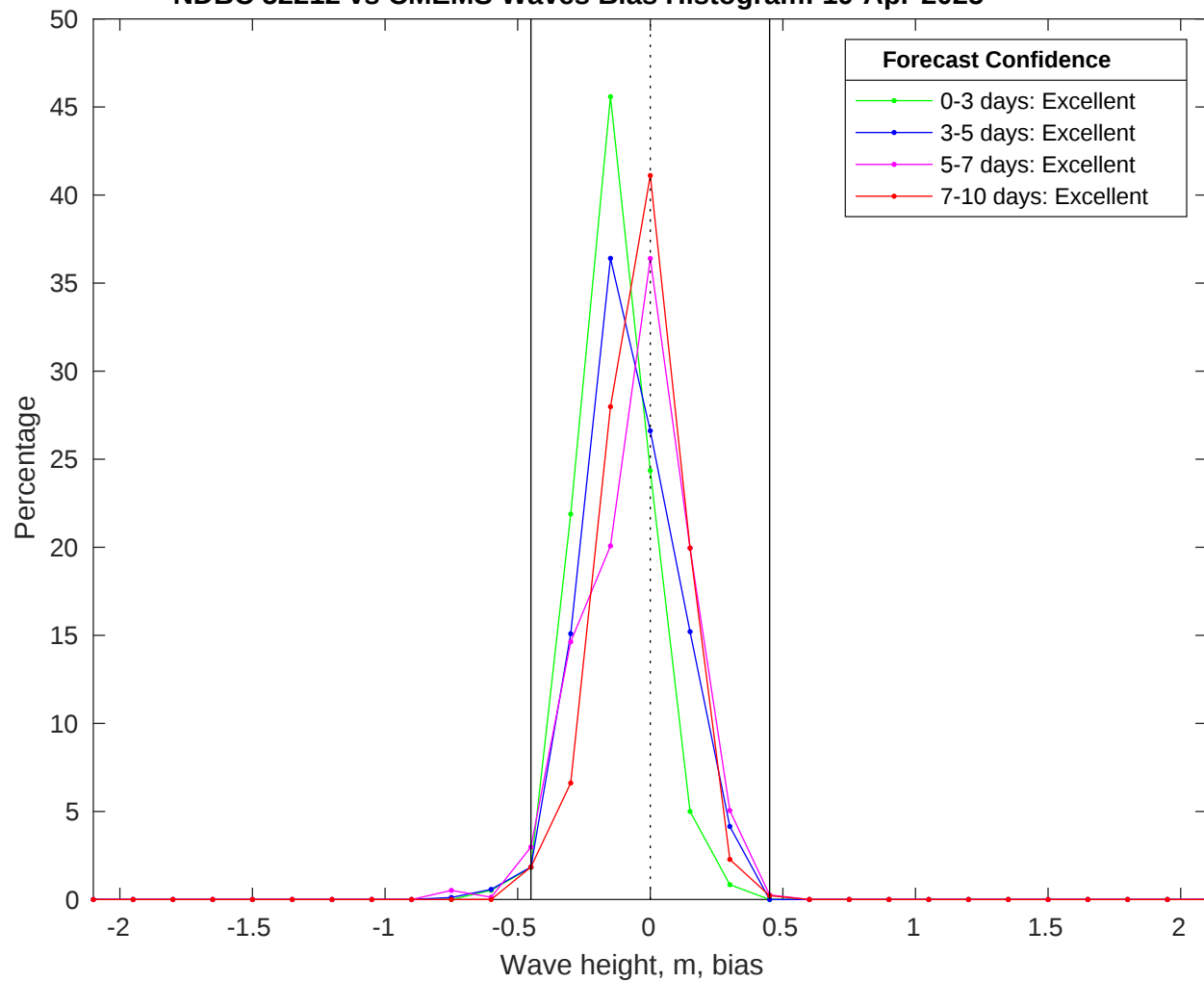
NDBC 52212 vs CMEMS Waves Bias Histogram: 19-Apr-2025
