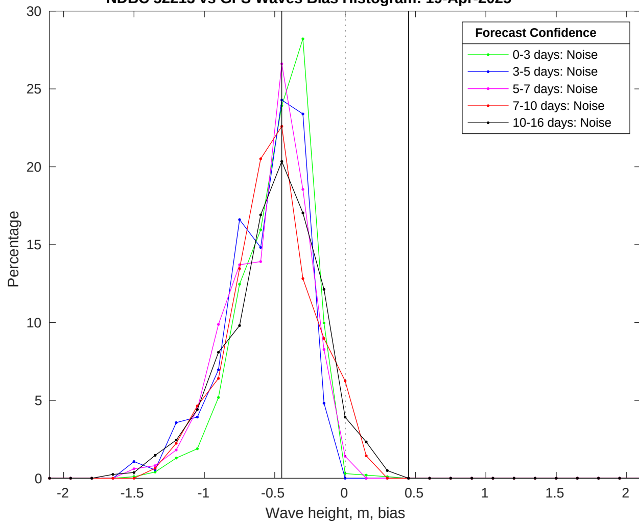
NDBC 52213 vs GFS Waves Bias Histogram: 19-Apr-2025
